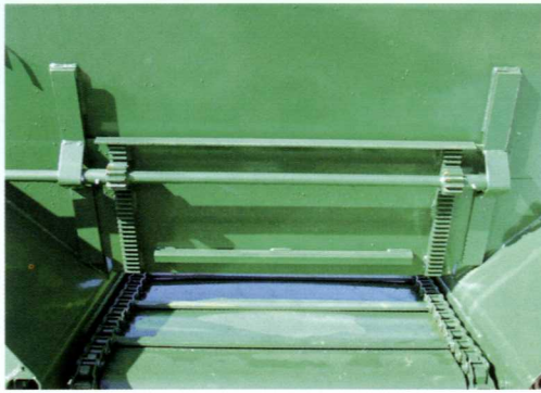
Rack & Pinion Gate For Jam-Free Operation
